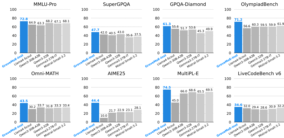
Figure 1: Benchmark performance of GroveMoE-Inst † and its counterparts. Our GroveMoE-Inst achieves performance comparable to open-source SOTA LLMs of similar or even larger scales.
