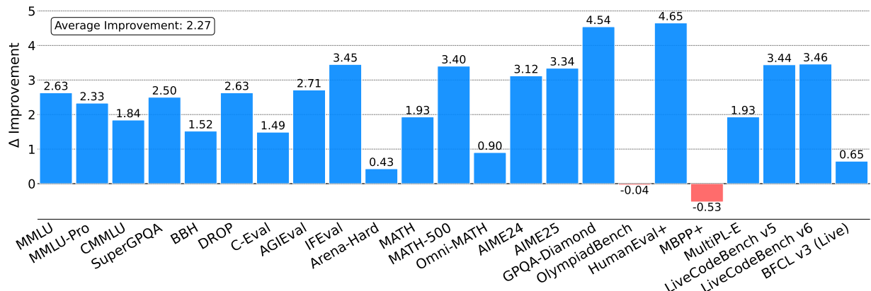
Figure 4: Evaluation results of SFT on various benchmarks. \Delta indicates the performance improvement of SFT trained with GroveMoE-Base over Qwen3-30B-A3B-Base.
