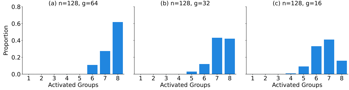
Figure 3: The group routing distribution across three configurations with different group numbers g . As the number of groups decreases, the average number of adjudgate experts activations decreases.
