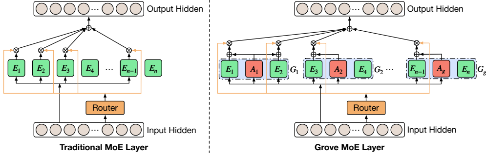
Figure 2: Comparison between the traditional MoE layer and our Grove MoE layer with dynamic computation allocation. For clarity, we configure n/g = 2 and k = 4 for the Grove MoE layer.
