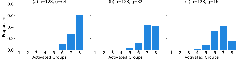
Figure 3: The group routing distribution across three configurations with different group numbers g . As g decreases, the average number of adjugate experts activations decreases.
