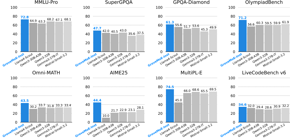
Figure 1: The performance of GroveMoE-Inst and its counterparts. GroveMoE-Inst achieves performance comparable to open-source SOTA LLMs of similar or even larger scales.
